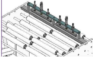
Bag Attachment Device
